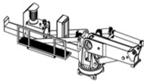
H 18 R AYAK ŞASE / LEG CHASIS
