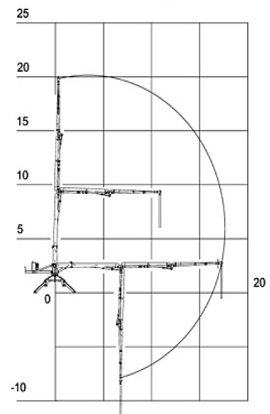
H 18 WORKING RANGE
